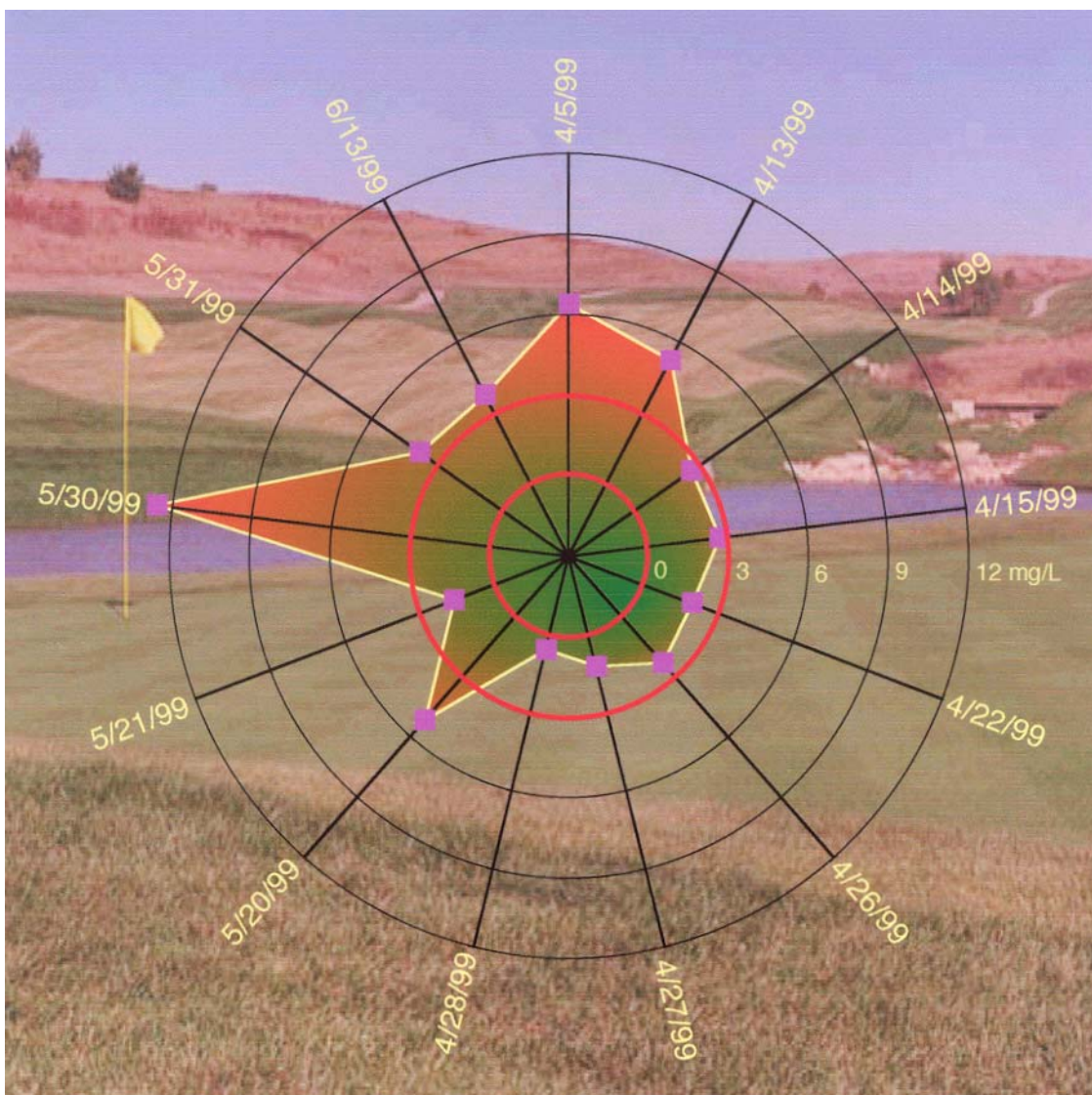
Figure 6. A spider radar graph displaying daily average of total nitrogen concentrations in runoff water on episodic days in April, May and June, 1999 where Little Kitten Creek exits Colbert Hills Golf Course. The upper control limit (larger red circle) is set at 3 \text{ mg L}^{-1} and the lower control limit (smaller red circle) is set at 0 \text{ mg L}^{-1} .
