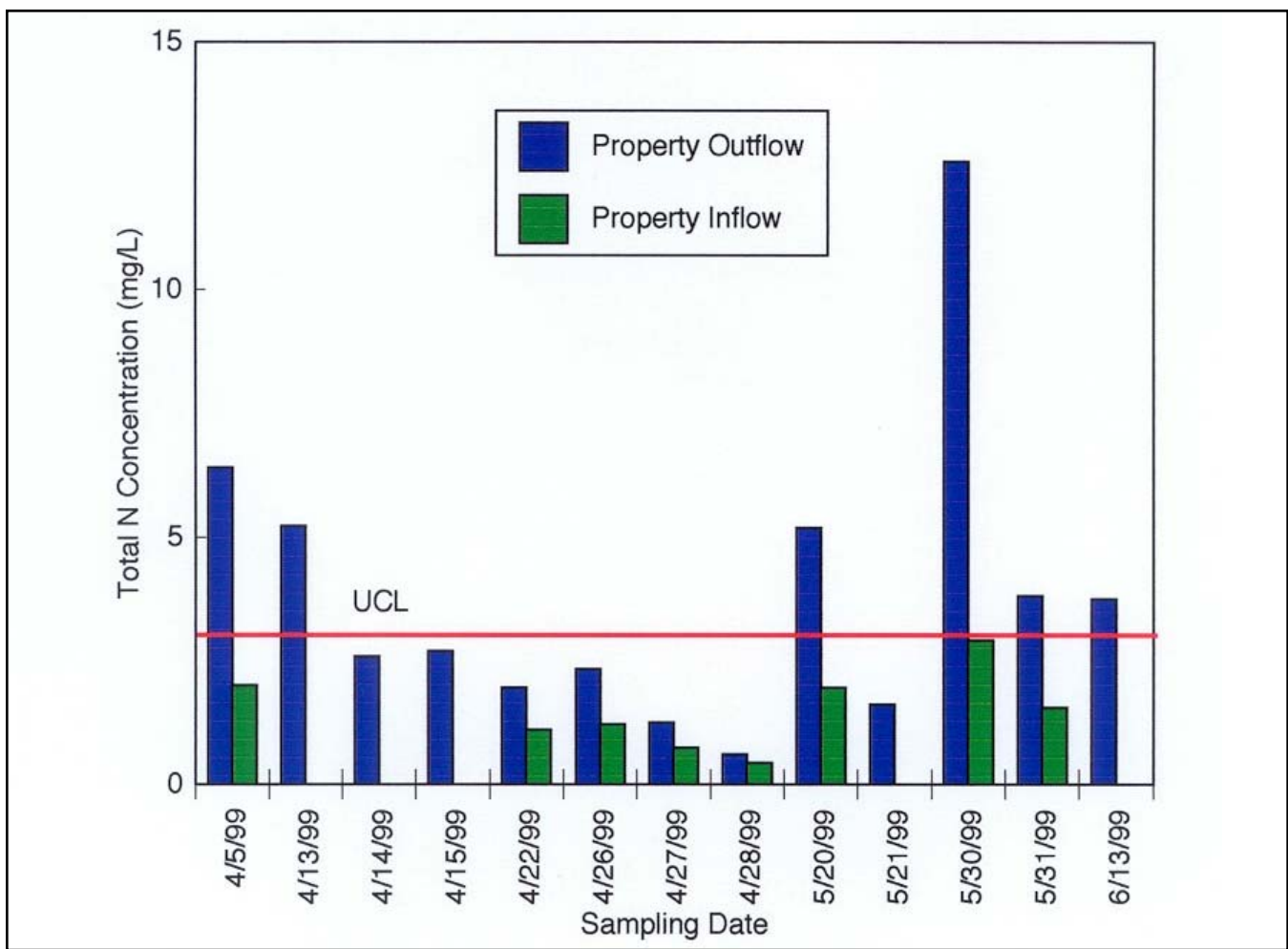
Figure 5. A control chart for daily average of total nitrogen concentrations in runoff water on episodic days in April, May, and June, 1999 for Little Kitten Creek where it exits and enters Colbert Hills Golf Course. The upper control limit (UCL) is set at 3 mg L -1 .
