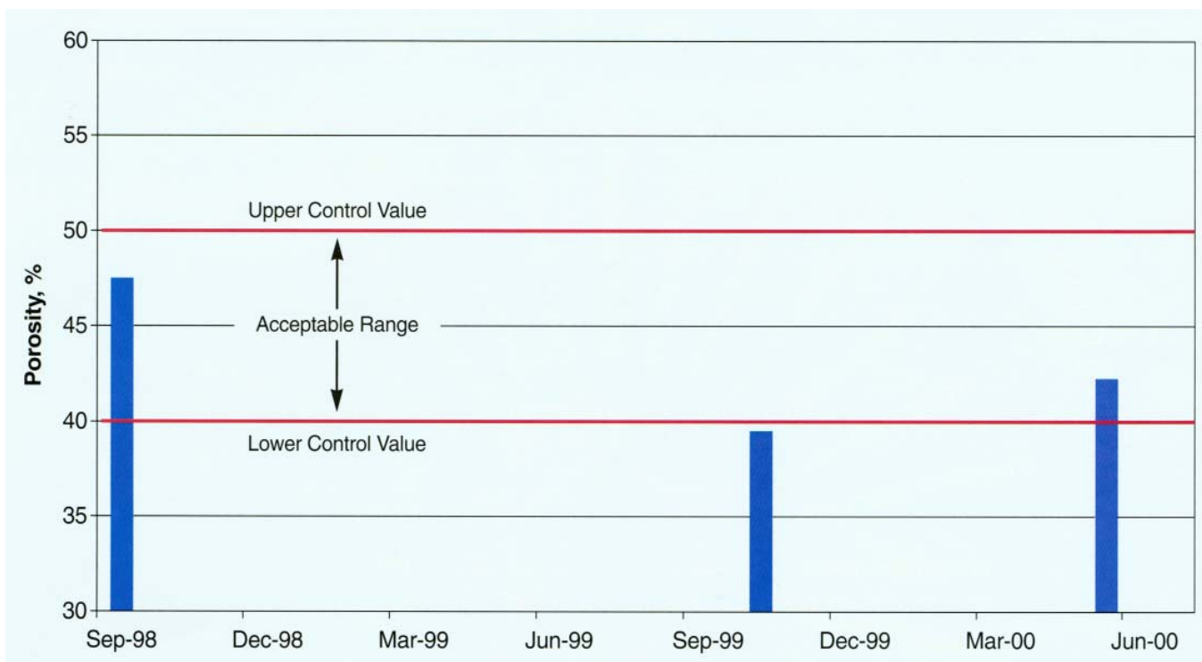
Figure 4. Control chart for soil porosity, an indicator of soil quality. Soil porosity was within the acceptable range prior to construction (Sep-98), but fell below acceptability during construction (Oct-99). Some sod establishment problems were evident. After one winter of freezing-thawing and wetting-drying, porosity returned to the acceptable range (May-00).
